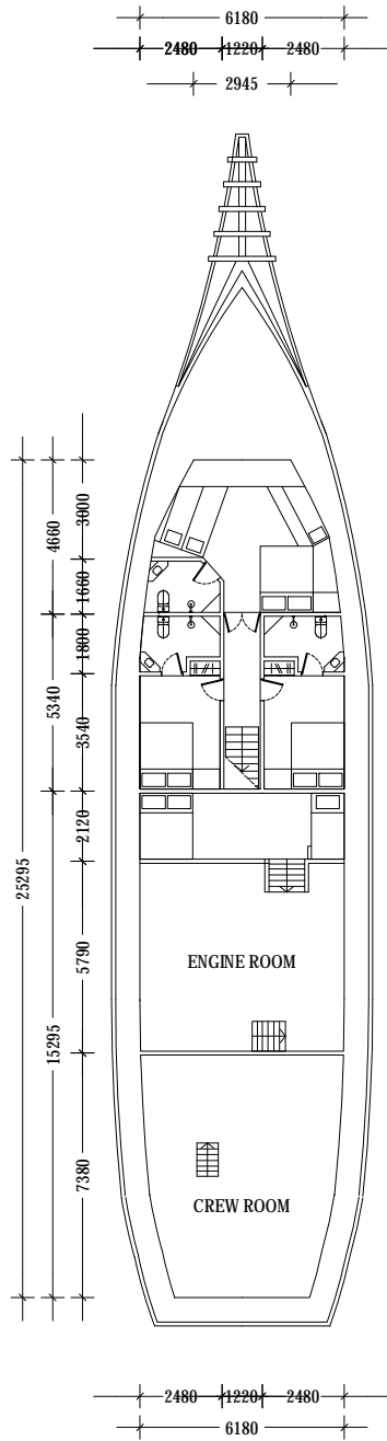
LEVEL 1 SCALE 1: 250
