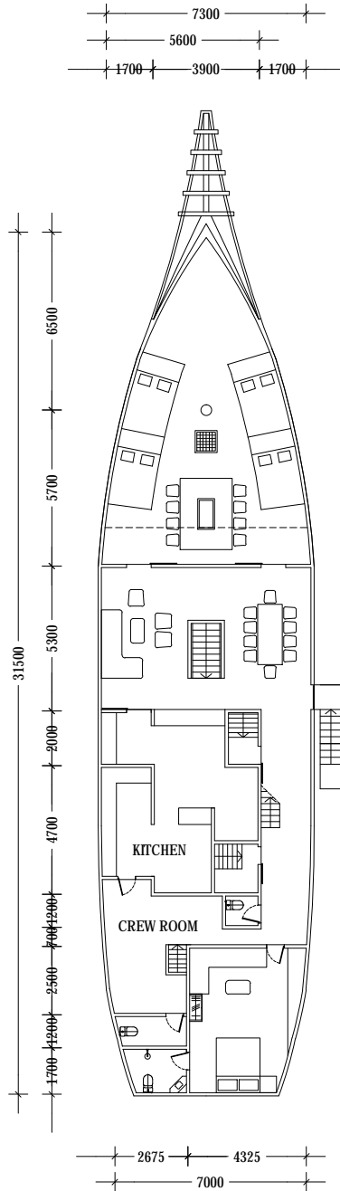
LEVEL 2 SCALE 1: 250
