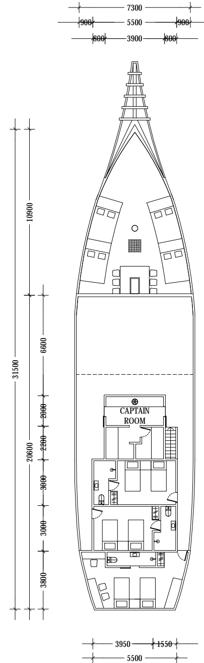
LEVEL 3 SCALE 1: 250
